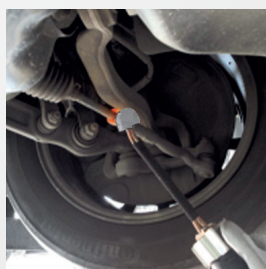
Releasing of steering linkage
